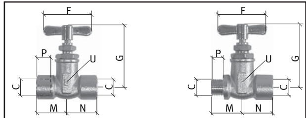
Muffe / Muffe
