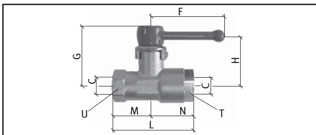
Muffe / Muffe
